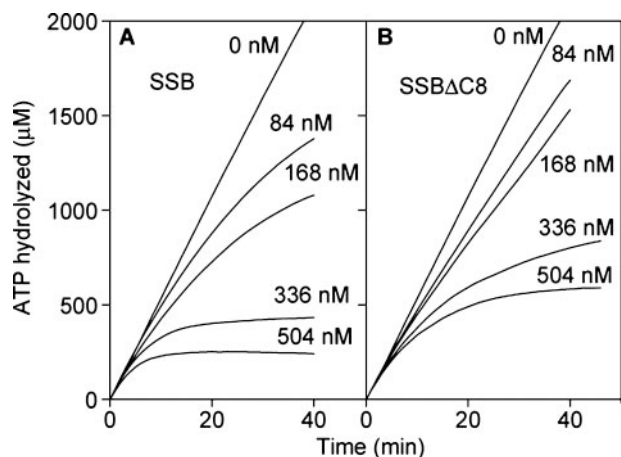
FIGURE 6. RecX protein can overcome the effects of SSB concentration. RecA, ssDNA, and ATP concentrations were identical to those in Fig. 2. SSB concentration was 1.8 \mu\text{M} . RecX protein concentration was varied as indicated. The SSB \Delta C8 protein used in panel B has a C-terminal truncation of eight amino acid residues that eliminates an interaction point used by multiple proteins in DNA metabolism. See text for details.
