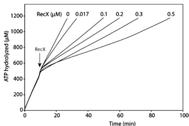
FIGURE 8. RecX inhibits RecA protein filaments bound to poly(dT). The poly(dT) and RecA protein concentrations were 4 and 2.4 \mu\text{M} , respectively. ATP was present at 3 \text{ mM} . RecX protein concentrations (in \mu\text{M} ) are indicated in the figure. RecA was incubated with poly(dT) and ATP and then challenged with the indicated concentration of RecX protein at the point denoted with the vertical arrow. The apparent small but abrupt increase in hydrolyzed ATP seen upon RecX addition is an artifact associated with the volume change accompanying the RecX addition.
