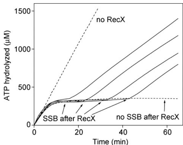
FIGURE 7. SSB can reverse the effects of RecX protein. RecA, ssDNA, and ATP concentrations were identical to those in Fig. 2. RecX concentration was 42 \text{ nM} . SSB protein was added at two different times. The first portion was added after RecA protein, at a concentration of 0.25 \mu\text{M} . The second addition (as indicated by an arrow) was added at various times thereafter, after RecX. The final concentration of SSB (total) was 3.5 \mu\text{M} . Time 0 corresponds to the time of the RecX addition.
