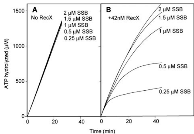
FIGURE 2. SSB protein antagonizes RecX function. The reactions were carried out as described under "Experimental Procedures" and contained 3 \mu\text{M} RecA protein, 5 \mu\text{M} M13mp8 ssDNA, 3 mM ATP, and (where indicated) 42 nM RecX. The SSB protein concentration was varied as indicated.
