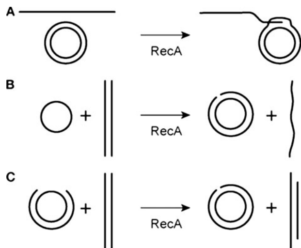
FIGURE 1. DNA pairing and strand exchange promoted by the RecA protein. Three typical reactions are shown. A , D-loop formation. The reaction involves the insertion of a linear single-strand DNA (or short oligonucleotide) into a duplex DNA, with a strand of the duplex displaced over the length of the paired inserted DNA. For highest yields, the duplex DNA is often a supercoiled circle. B , the three strand exchange reaction. C , the four-strand exchange reaction (initiated as a three-strand reaction in the gap of the DNA circle).
