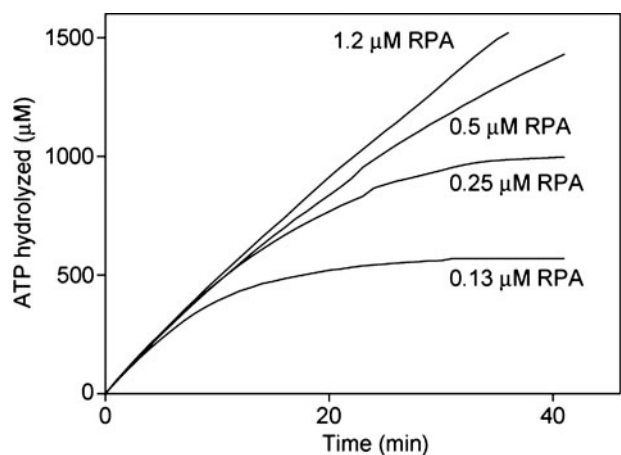
FIGURE 4. The protective effects of SSB are not species-specific. The reaction conditions were as in Fig. 2, but with RPA replacing SSB. RPA protein concentration was varied as indicated.
