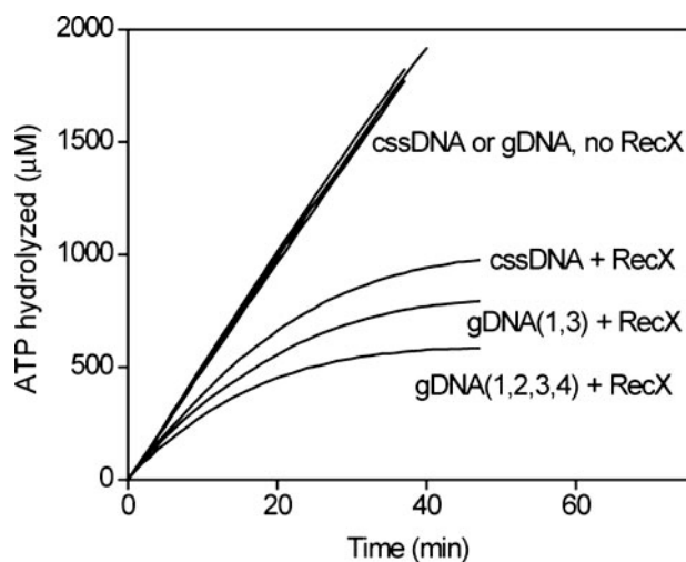
FIGURE 5. The protective effect of SSB is reduced on gDNA. RecA, ssDNA, and ATP concentrations were identical to those in Fig. 2. RecX concentration was 84 nM (where indicated). In all cases, the SSB was present at 1.5 μM.
