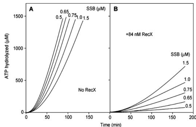
FIGURE 3. SSB and RecX were bound to the ssDNA prior to addition of the RecA. RecA, ssDNA, and ATP concentrations were identical to those in Fig. 2. RecX concentration was 84 nM (where indicated). The SSB concentration was varied. SSB and RecX protein (when present) were preincubated with the ssDNA and ATP during the 10 min prior to introduction of RecA protein. The RecA protein addition defines the zero time point.
